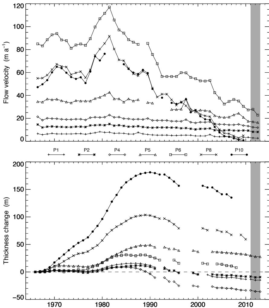
Figure 6.3: Surface flow velocities (top) and thickness change (bottom) of the Glacier du G etro at all 7 stakes. Note the gaps that hamper the interpretation of the total thickness change. The gray shaded area highlights the years of the current report.
