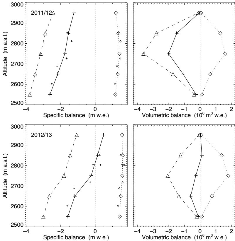
Figure 4.26: Glacier de Tsanfleuron - Specific (left) and volumetric (right) winter (dotted, \diamond ), summer (dashed, \triangle ) and annual (continuous line, +) balance versus altitude for 2011/12 (top) and 2012/13 (bottom). Small symbols mark the individual measurements.
