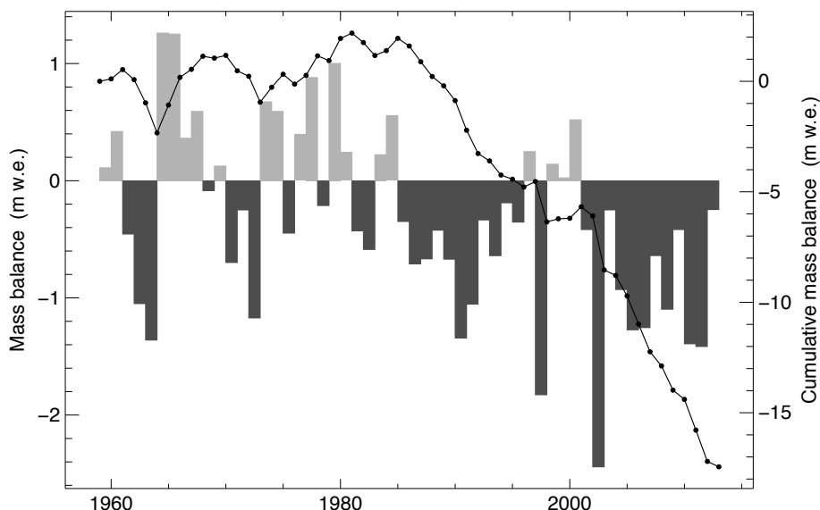
Figure 4.22: Silvrettagletscher - Mean specific annual balance (bars) and cumulative mass balance (line) for the period 1959-2013.
