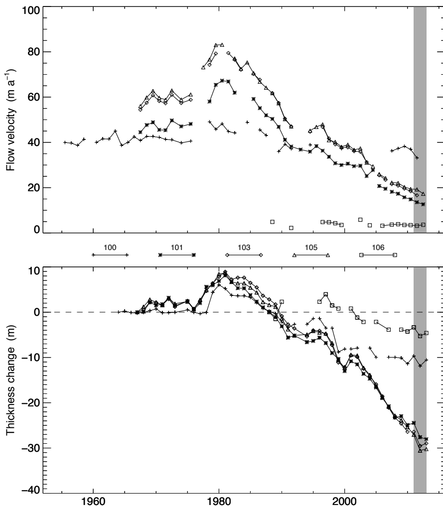
Figure 6.9: Surface flow velocities (top) and thickness change (below) of the Allalingsgletscher at 5 stakes. The gray shaded area highlights the years of the current report.
