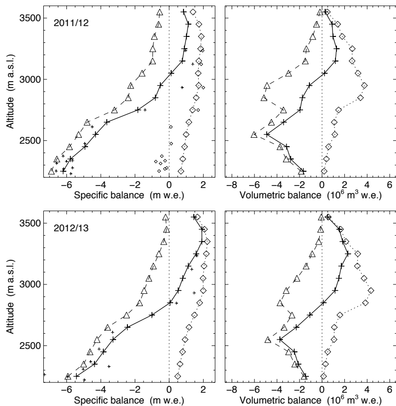
Figure 4.18: Specific (left) and volumetric (right) winter (dotted, \diamond ), summer (dashed, \triangle ) and annual (continuous line, + ) balance versus altitude for 2011/12 (top) and 2012/13 (bottom). Small symbols mark the individual measurements.
