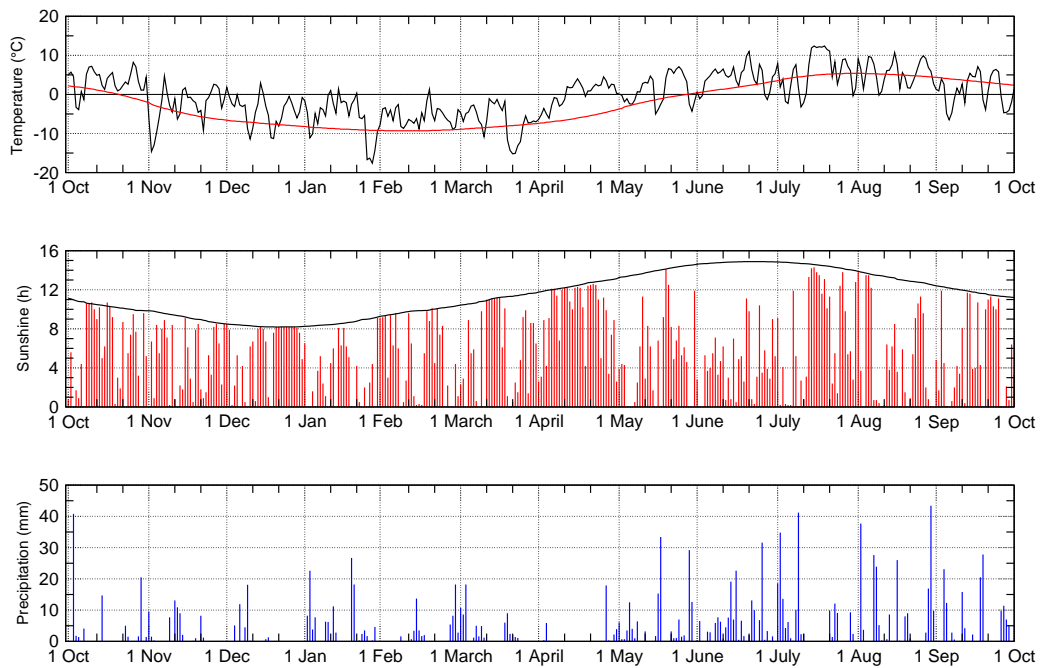
Figure 2: Daily meteorological conditions at Weissfluhjoch for the reporting period 2006/07. top: temperature (black) with long-term mean values (red), center: sunshine duration (red) with theoretical maximum (black), bottom: daily precipitation totals (blue) .
