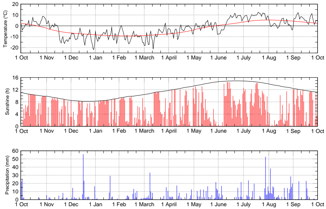
Figure 1: Daily meteorological conditions at Weissfluhjoch for the reporting period 2005/06. top: temperature (black) with long-term mean values (red), center: sunshine duration (red) with theoretical maximum (black), bottom: daily precipitation totals (blue) .
